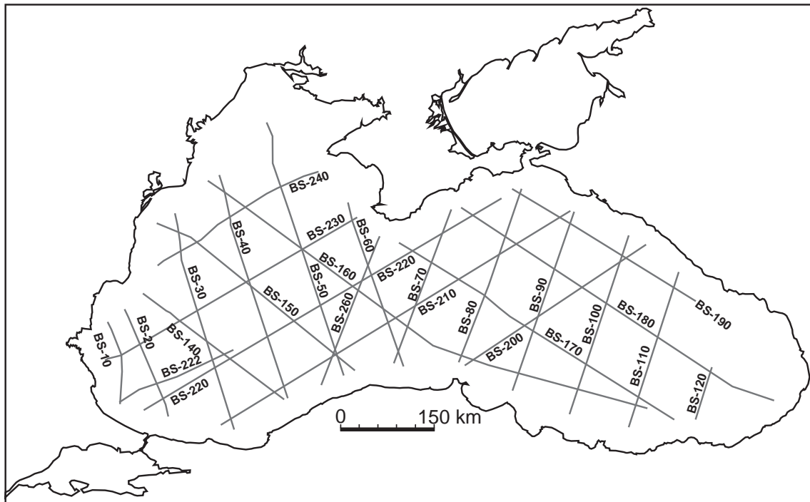
Figure 2. Location of the seismic lines presented in this paper. The seismic lines were acquired in 2011 within the framework of “Geology Without Limits” project.
