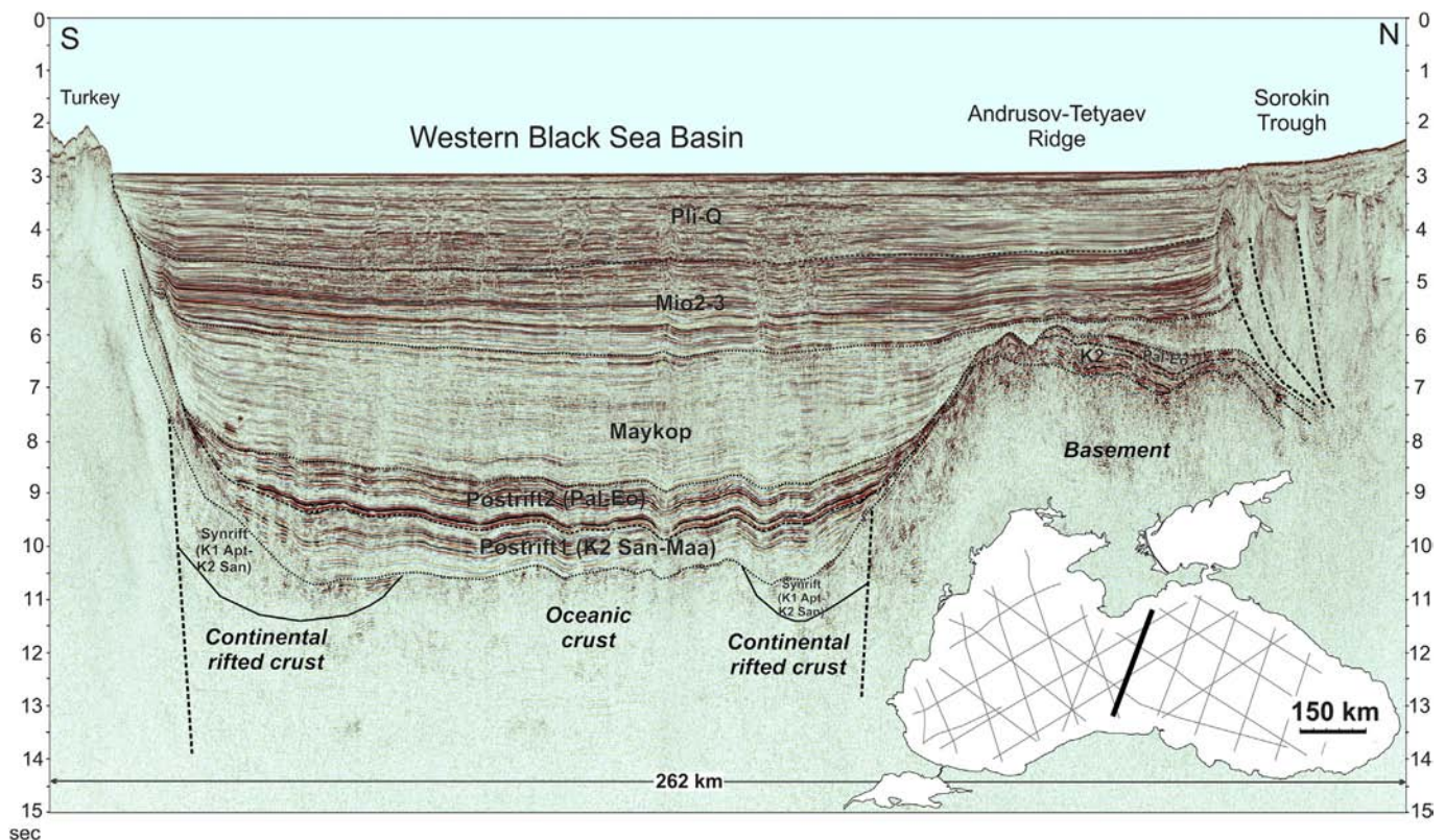
Figure 8. Geological interpretation of seismic line BS-70. The Andrusov-Tetyaev Ridge is a continental block. The Sorokin Trough is the Maykopian flexural foredeep basin for the South Crimea Orogen. The Andrusov-Tetyaev Ridge is tilted toward the Sorokin Trough as a peripheral bulge. The Sorokin Trough was folded during Neogene times. The fold structure is bounded by detachment surfaces at the bottom of the Maykop sequence.
