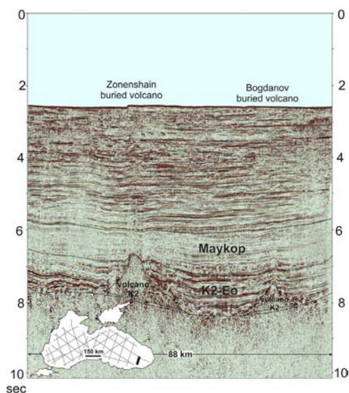
Figure 11. Geological interpretation of seismic line BS-120. Two possible Late Cretaceous volcanoes could be interpreted in this line; they are located in the Trabzon Basin not far from the Pontide Cretaceous volcanic belt.
