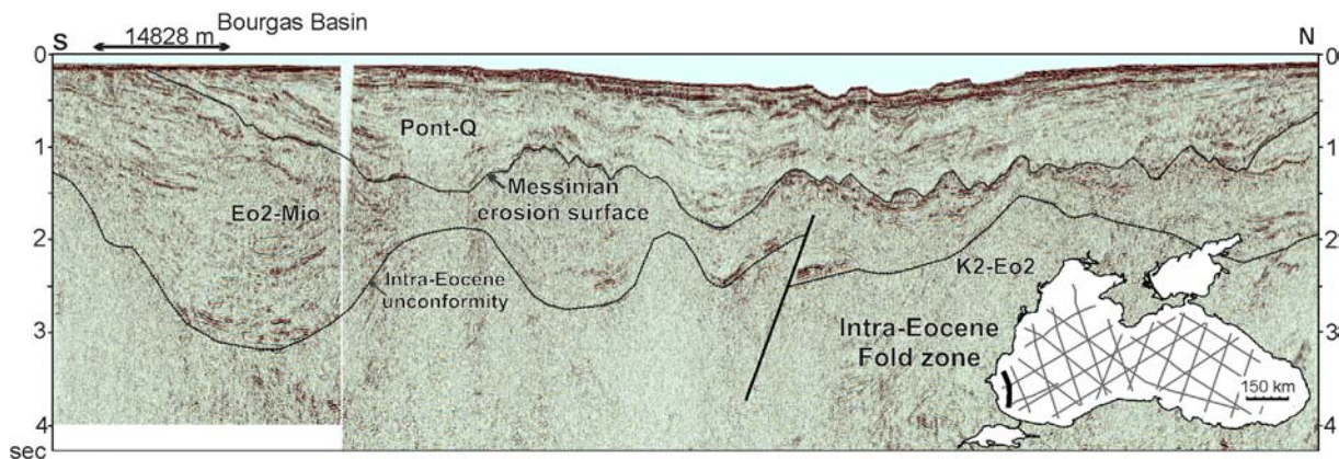
Figure 3. Geological interpretation of seismic line BS-10. Two erosional surfaces are easily identifiable in this profile. We interpret the upper one as the Messinian erosion surface, which originated due to a rapid sea level fall ( Suc et al., 2011 ; Munteanu et al., 2011, 2012 ; Bache et al., 2012 ); the deeper erosional surface corresponds to the intra-Eocene unconformity. Pont – Pontian, Eo – Eocene, K – Cretaceous. For location of this and other lines see Figure 2 .
