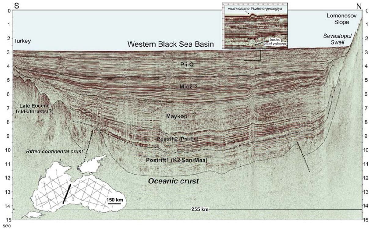
Figure 20. Geological interpretation of seismic line BS-260. This line shows some structure of the Western Black Sea Basin. The Sevastopol Swell possibly corresponds to a transpressional structure. A recent, active mud volcano is recognized as a positive structure on the sea bed; at depth, a buried mud volcano system is seen, with roots in the Maykopian stratigraphic level.
