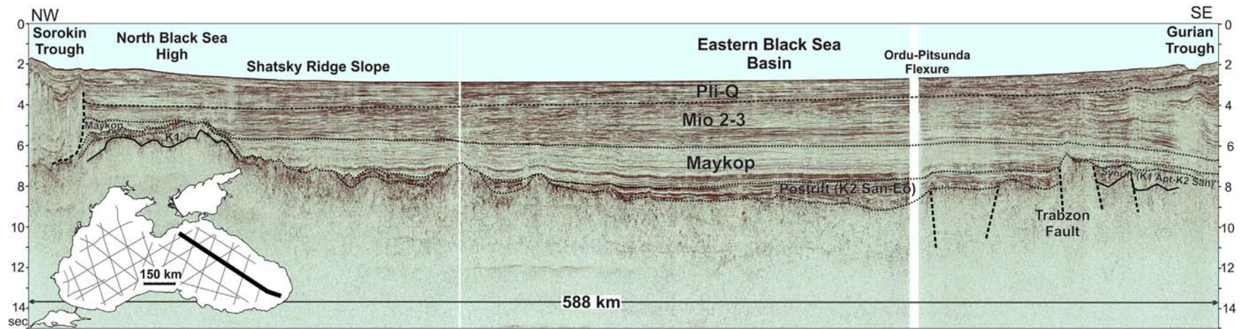
Figure 14. Geological interpretation of seismic line BS-180. This line follows the axis of the Eastern Black Sea Basin. The North Black Sea High, one of the highest uplifts of the Shatsky Ridge, was a tilted block during Maykopian times and acted as a peripheral bulge simultaneously for the Sorokin and Tuapse foredeep flexural basins. The Ordu–Pitsunda Flexure separates the Eastern Black Sea and the Trabzon basins. The Gurian Trough has no anomalously thick Maykopian deposits as compared with the Tuapse and Sorokin troughs. The Gurian Trough is possibly Miocene in age and it is not analogous to the Tuapse and Sorokin troughs.
