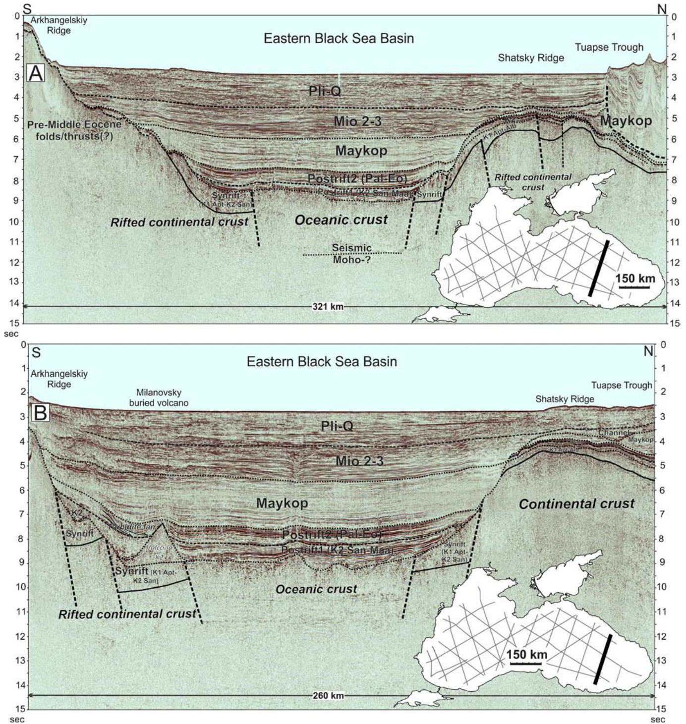
Figure 10. A. Geological interpretation of seismic line BS-100. The Eastern Black Sea looks like a nearly symmetric rift basin. B. Geological interpretation of seismic line BS-110. Top of the crustal basement in the central part of the Eastern Black Sea Basin has a hummocky structure, possibly indicating the presence of volcanic bodies or tilted fault blocks. We interpret this surface as marking the top of the oceanic crust. A large mountain-like buried structure is located close to the Arkhangelskiy Ridge, which is also recognized perpendicularly on seismic line BS-170 (Fig. 13). On both lines the geometry of the structure is a cone-like buried mountain, leading us to interpret it as a Late Cretaceous volcano, with its base resting within postrift deposits. The volcano shows no signs of erosion features at its top, and it is buried by sediments of possible Eocene age. We conclude that the volcano originated in a deep-water Late Cretaceous basin, where water depth could be in excess of 2–3 km (1.5 s seismic time). The volcano is located slightly to the north of the Pontides Cretaceous volcanic belt in Turkey.
