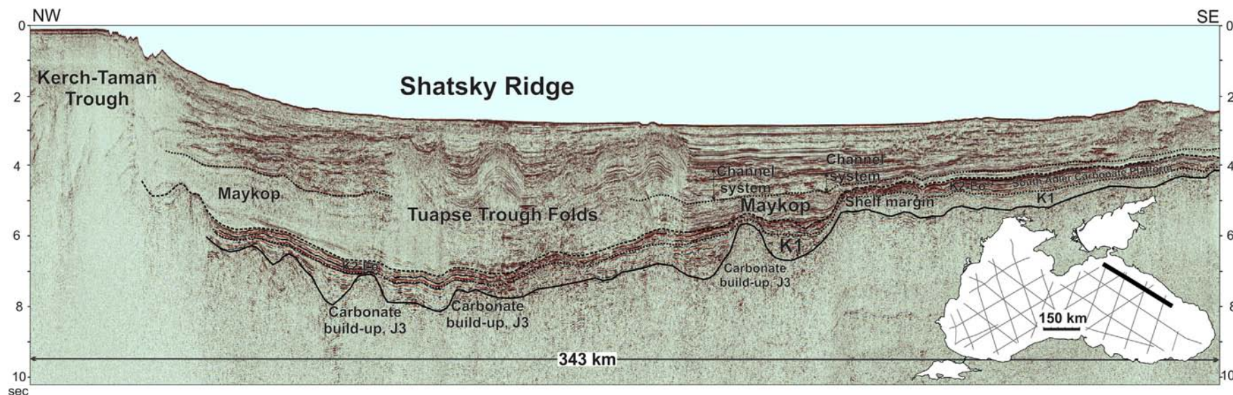
Figure 15. Geological interpretation of seismic line BS-190. The profile follows the axis of the Shatsky Ridge. The northern part of the Shatsky ridge is different from its southern part. The large South Adler platform characterizes its southern part; it is likely composed of Upper Jurassic to Eocene shallow marine carbonates. Large Late Jurassic carbonate build-ups are recognized on the northern part of the Shatsky Ridge (Afanasenkov et al., 2007; Nikishin et al., 2012). J3 – Upper Jurassic.
