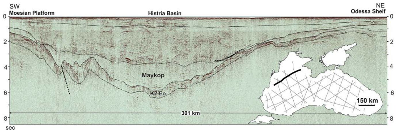
Figure 19. Geological interpretation of seismic line BS-240. This line shows the structure of the Histria Basin, which was effected by inversion tectonics during the Late Eocene to Oligocene. It was rapidly filled by Maykopian to Recent deposits.
