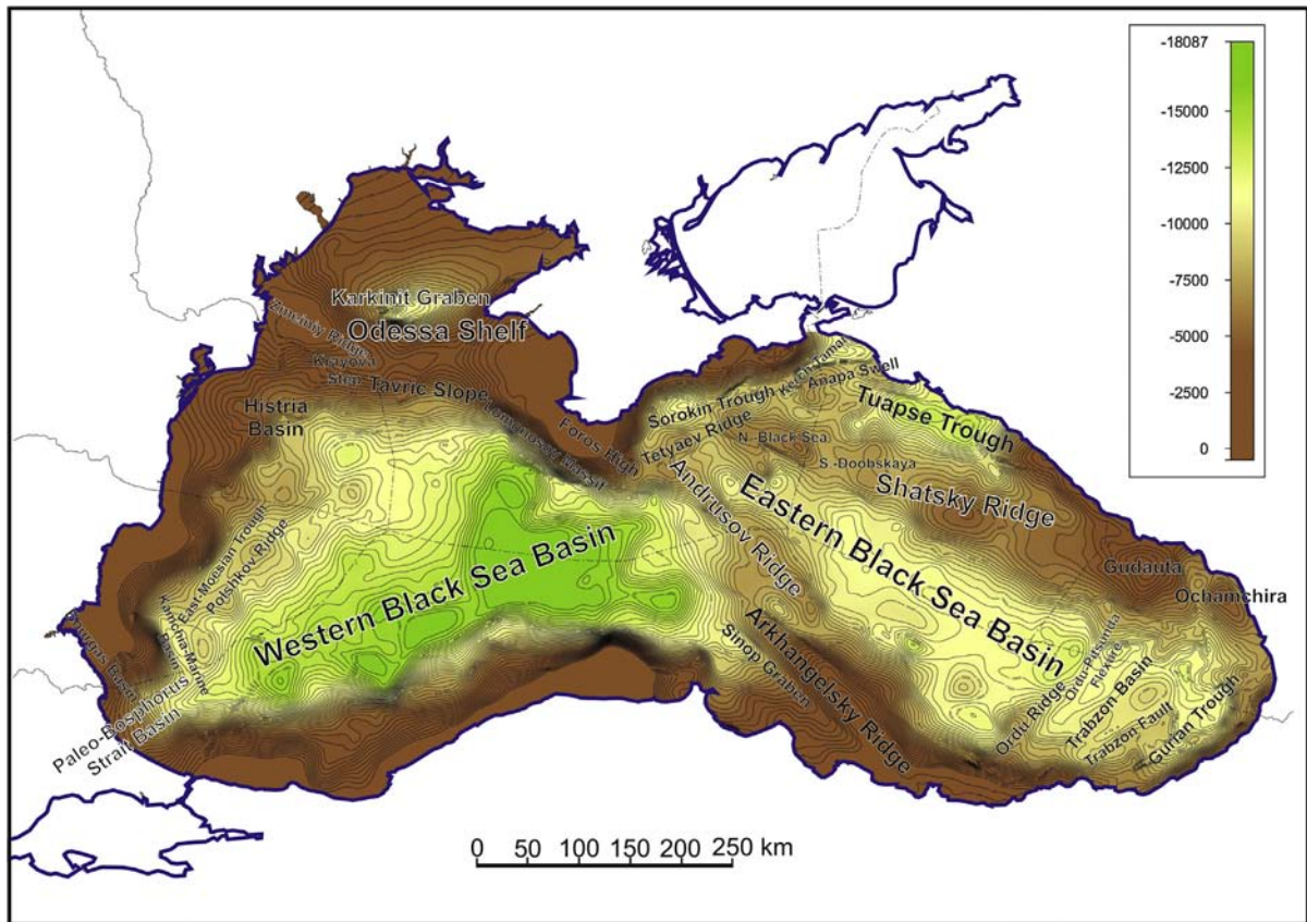
Figure 21. Basement topography of the Black Sea Basin. This map is based mainly on data from the new seismic lines.
