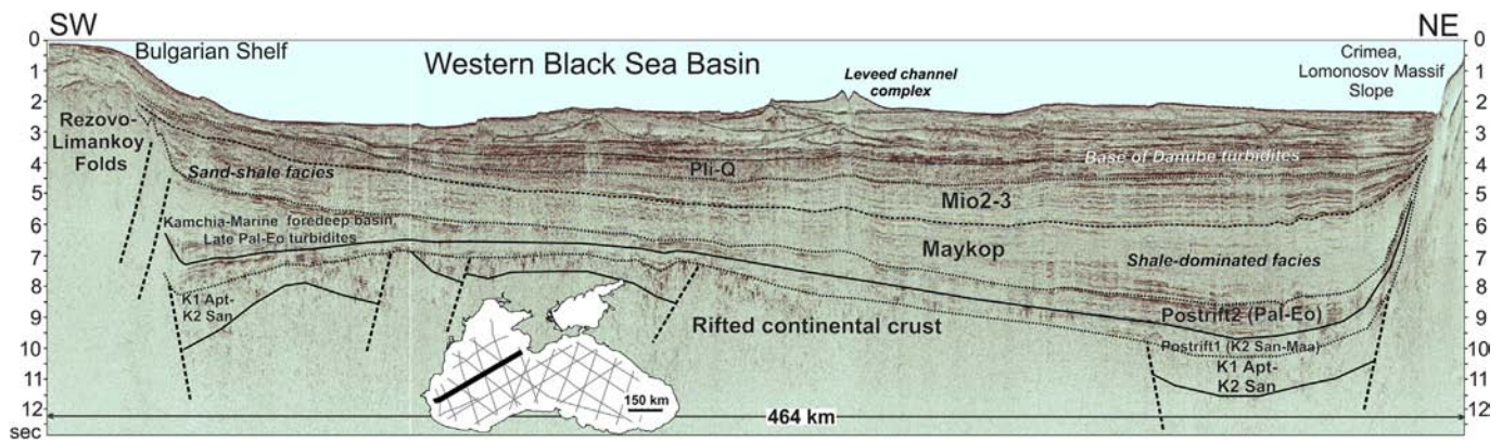
Figure 18. Geological interpretation of seismic line BS-230. Some graben-like structures are seen below the post-rift regional cover. A large sedimentary wedge of approximately Paleocene–Eocene age (pre-Maykopian) is seen close to the Bulgarian Shelf; it is interpreted as a flexural foredeep basin. This basin is probably the offshore continuation of the Kamchia Foredeep Basin of Late Paleocene–Middle Eocene age, well described in Bulgaria (Tari et al., 2009; Stuart et al., 2011; Georgiev, 2012). Large leveed channel complexes are seen between the Bulgarian and the Crimea continental slopes. The base of this complex lies close to Miocene/Pliocene boundary; according to the interpretation of this seismic line, the origin of the Danube Delta is close to the Messinian erosion event.
