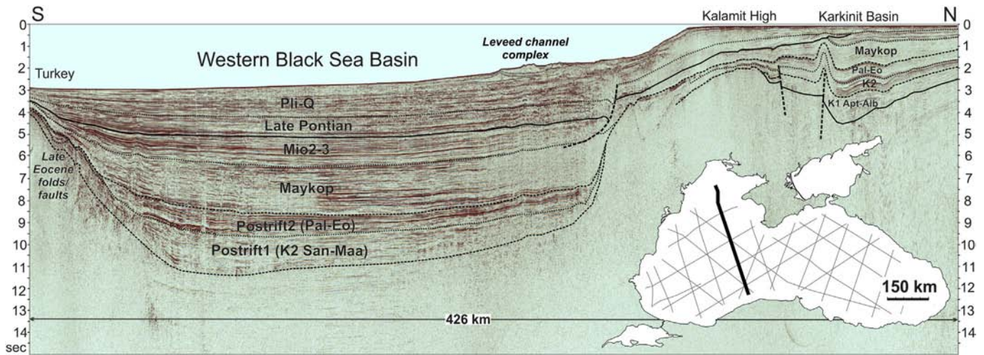
Figure 6. Geological interpretation of seismic line BS-50. The leveed channel complex of the distal Danube fan system is distinctly recognizable. The Late Pontian unit is interpreted as a sequence deposited immediately after the Messinian erosion event. The Karkinit Basin is a rifted basin partly inverted during the Late Eocene to Oligocene time.
