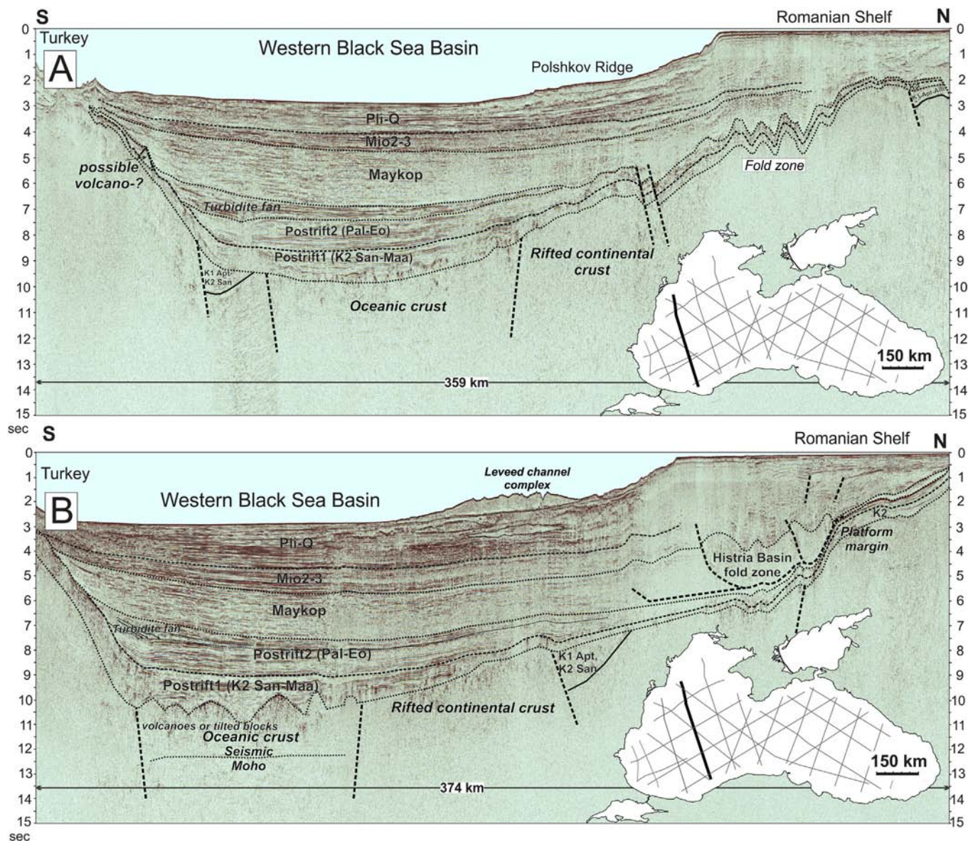
Figure 5. A. Geological interpretation of seismic line BS-30. The Romanian Shelf is characterized by a thick Oligocene to Recent sedimentary sequence. Late Eocene to Oligocene inversion structures (Dinu et al., 2005; Munteanu et al., 2011) are clearly recognizable. The Polishkov Ridge is bounded to the northwest by possible normal or transtensional faults of Oligocene age. A large Upper Eocene turbidite unit was possibly fed by the uplift of the Western Pontides (Istanbul Terrane). The Western Black Sea Basin has a general asymmetric geometry; the southern slope is very steep while the northern slope is gentler and have some internal steps. B. Geological interpretation of seismic line BS-40. The leveed channel complex of the distal Danube fan-delta (Lericolais et al., 2010; Munteanu et al., 2012) is well recognizable. The Histria Basin in the Romanian Shelf has a complicated structure including gravity-driven thrusting and folding. A large turbidite unit is seen at the Upper Eocene level, possibly related with the Late Eocene uplift of the Western Pontides (Istanbul Terrane). A considerable part of the top of the acoustic basement in the basin has a characteristic hummocky surface with lense-shaped sediment infill. Such relief is probably caused by extension of the lithosphere and irregular filling of linear zones with volcanic material. The general asymmetry of the basin is well expressed: the southern slope is steep and the northern slope is much gentler.
