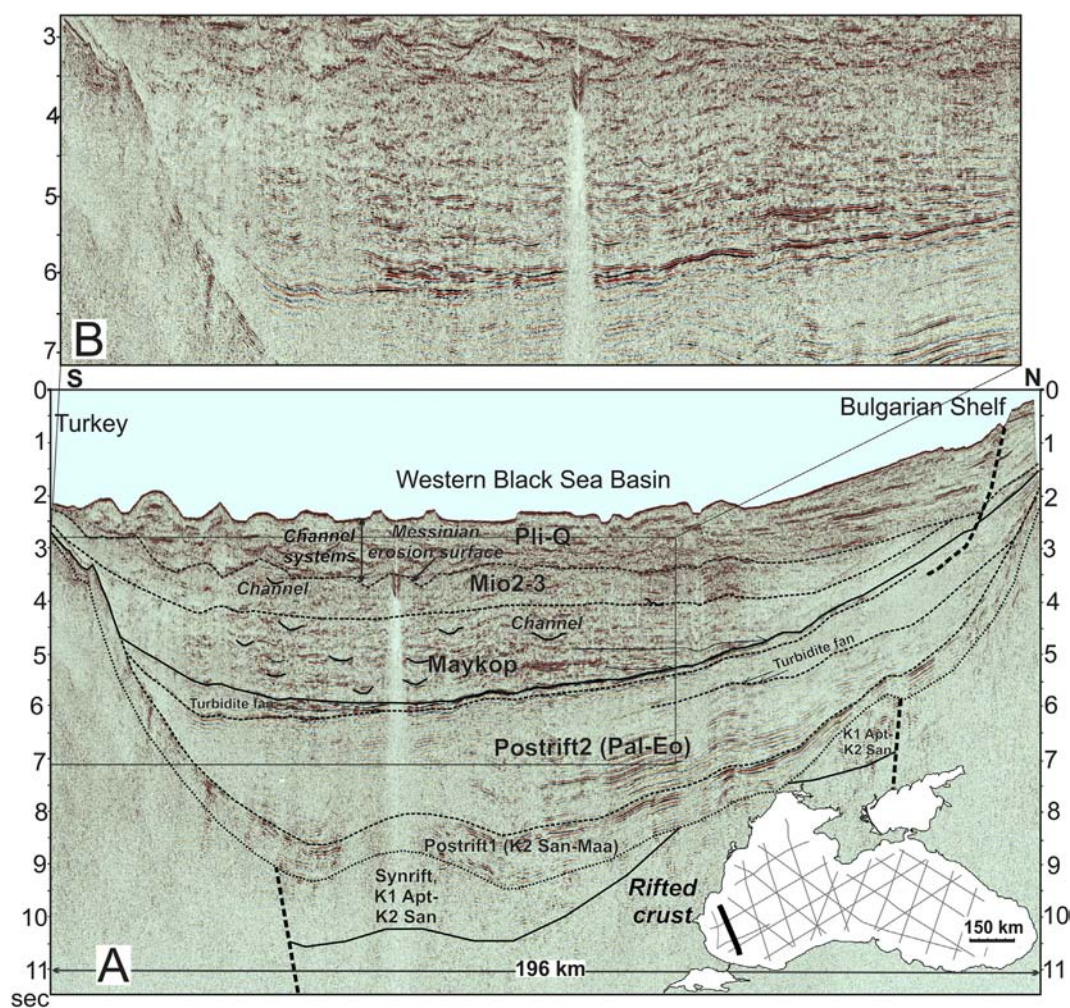
Figure 4. A. Geological interpretation of seismic line BS-20. The Messinian erosion surface is well expressed. The Maykopian seismocomplex is characterized by a number of channel features. We suggest that transport of clastic material was from the Thrace Basin in the Balkans. Turbidite fans are interpreted at the uppermost part of the Eocene sequence, which originated possibly from an uplift of the Western Pontides (Istanbul Terrane) and Balkanides. Half-graben like structures are likely present at the base of the sedimentary sequence. A rift-related origin of the basin is most probable (Finetti et al., 1988; Robinson et al., 1996; Nikishin et al., 2003, 2012). Pli – Pliocene, Q – Quaternary, Mio – Miocene, Apt – Aptian, San – Santonian, Maa – Maastrichtian. B. Un-interpreted window of the seismic section.
