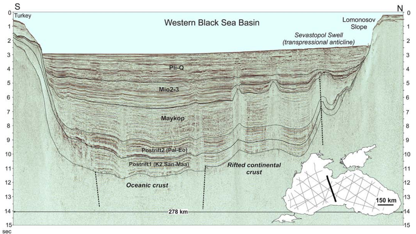
Figure 7. Geological interpretation of seismic line BS-60. The Lomonosov Slope consisting of Albian, Middle Jurassic and possible Paleozoic and older rocks (Shnyukov et al., 1997) is a basement for the Black Sea sedimentary cover. Middle Jurassic (Bajocian) age ( 168 \pm 1.7 Ma) of volcanics was recently obtained using zircon dating (Shnyukova, 2013). Based on this seismic line, we identify the Sevastopol Swell as a Neogene structure possibly originating from transpressional movements along the former rifted passive margin.
