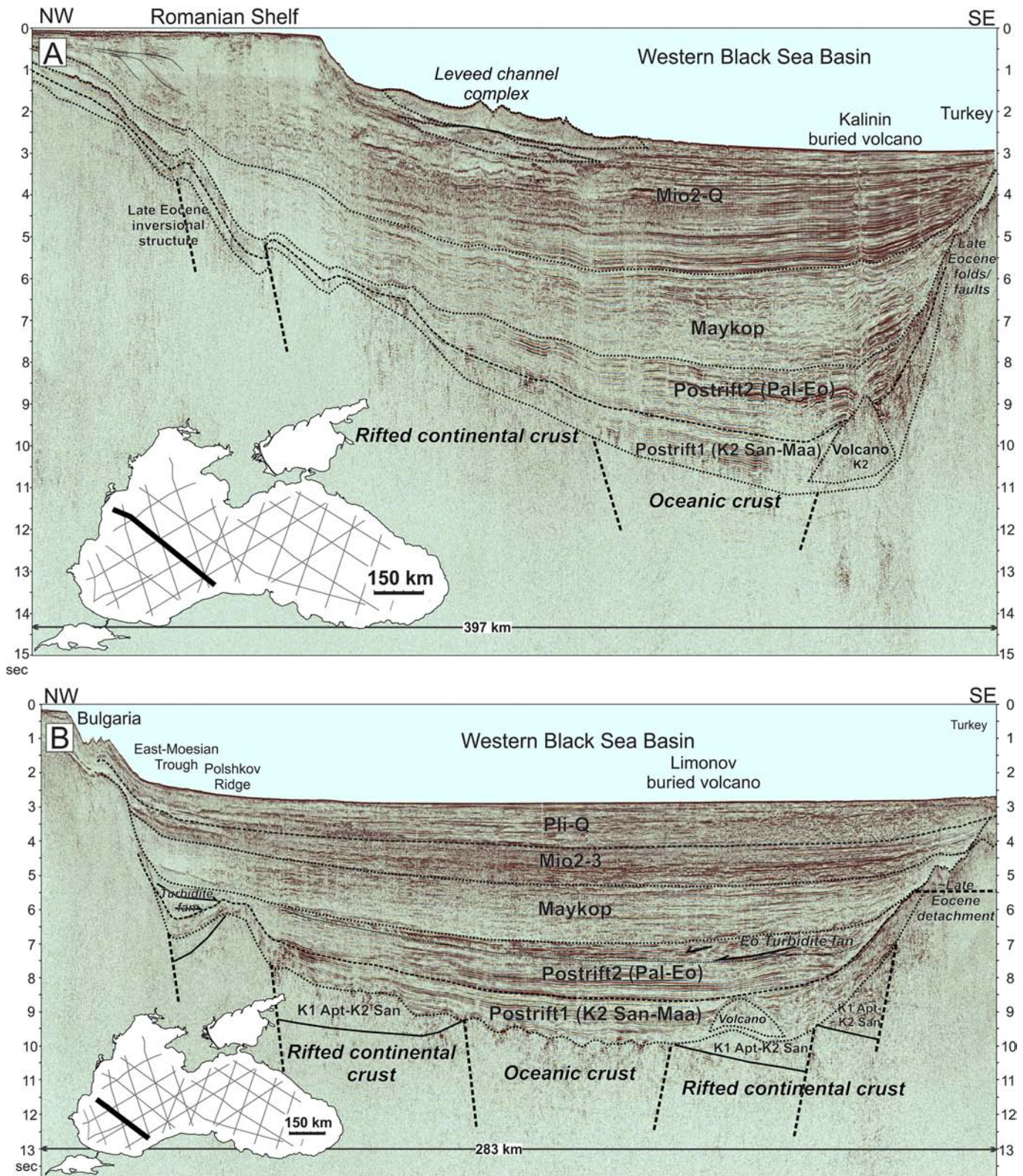
Figure 12. A. Geological interpretation of seismic line BS-150. The Western Black Sea is an asymmetric rift basin. The Romanian Shelf has a thick sedimentary sequence. Late Eocene to Oligocene inversion structures are typical for this shelf. A buried possible Cretaceous volcano and a Neogene to Recent leveed channel complex are also distinguishable on this line. B. Geological interpretation of seismic line BS-140. This line crosses the East-Moesian Trough and the Polshkov Ridge in the Bulgarian sector of the Black Sea. A deeply buried Cretaceous volcano is mapped on the rifted continental crust of the Turkish sector. A turbidite fan fed by the Western Pontides is tentatively interpreted at the upper part of the Eocene sequence. The Western Pontides were folded and thrust toward the Black Sea during Late Eocene to Early Oligocene times (Okay et al., 2001; Sunal and Tüysüz, 2002; Cavazza et al., 2011). This fold and thrust belt is separated by a detachment surface at the bottom (Sunal and Tüysüz, 2002). We cannot see this fold and thrust structure on our seismic lines but the Maykopian deposits cover this fold and thrust belt and the proposed detachment surface.
