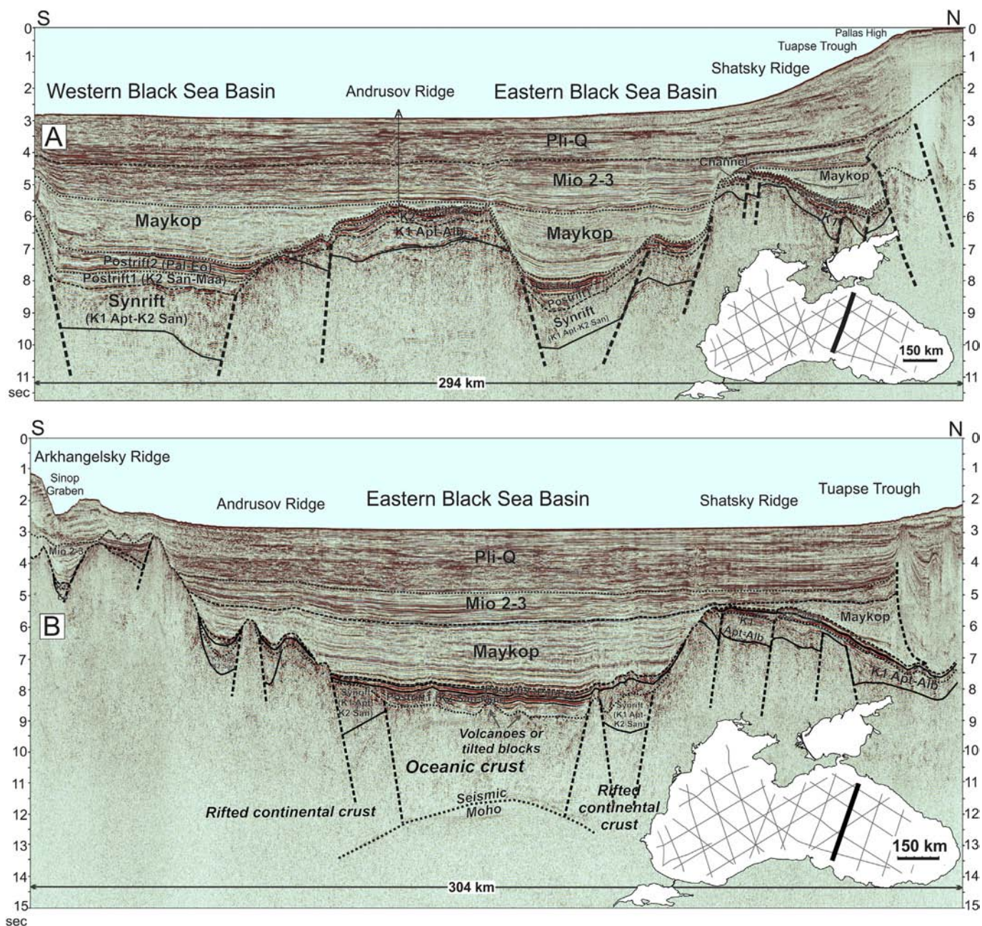
Figure 9. A. Geological interpretation of seismic line BS-80. The main features of the Black Sea Basins are well recognizable on this line. The Eastern Black Sea is a rifted Cretaceous basin. Details of the synrift geometry are not seen clearly on this line. The postrift sequence could be subdivided into a few units. The Western Black Sea Basin is similar to the Eastern basin, but here also the synrift structures are not seen in details. The Andrusov Ridge is a typical continental terrane with a sedimentary cover consisting of synrift and postrift sequences. The Andrusov and Shatsky ridges are very similar with respect to the basement and pre-Maykopian deposits. The Shatsky Ridge was tilted during the Oligocene as a peripheral bulge for the Maykopian Tuapse flexural foredeep basin. Post-Maykopian deposits commonly cover all the Black Sea Basins. The Shatsky and Andrusov ridges experienced marine sedimentation during Maykopian times, without any evidence of erosion. B. Geological interpretation of seismic line BS-90. A seismic reflector, possibly corresponding to the Moho is identified on this line. Seismic thickness of the oceanic crust is about 3–4 s. Rifted structure with Early Cretaceous normal faults is typical for the Shatsky and Andrusov ridges. The Tuapse Trough looks like a classical Maykopian flexural foredeep basin.
