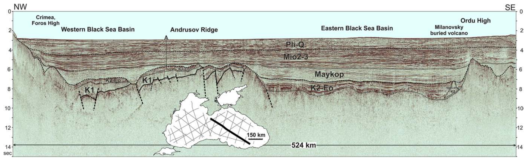
Figure 13. Geological interpretation of seismic line BS-170. The Andrusov Ridge is made up of a large continental block. Early Cretaceous half-grabens and normal faults are clearly identifiable. In our interpretation, the postrift cover consists of Upper Cretaceous sediments. The Ordu High is a continental block with no identifiable Mesozoic sedimentary cover.
