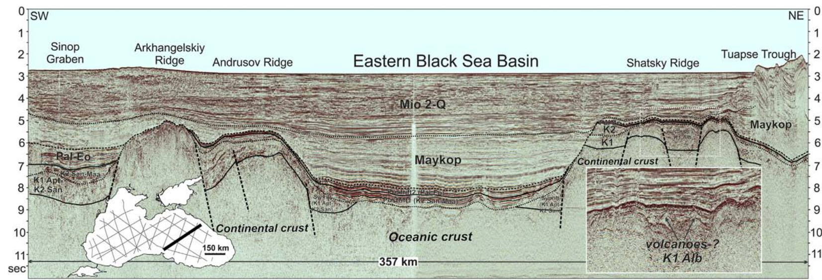
Figure 16. Geological interpretation of seismic line BS-200. The profile originates in the Tuapse Trough, crosses the Shatsky Ridge and the Eastern Black Sea Basin, the Andrusov and Arkhangelsky ridges and terminates in the Sinop Graben of the Western Black Sea Basin. The Shatsky Ridge has Early Cretaceous graben-like structures. One of these structures is characterized by hummocky seismic facies (see zoomed-in fragment of the profile within the inset). Height of some hummocks is up to 0.2–0.4 s. The corresponding regional stratigraphic level of this hummocky facies is approximately Albian. We therefore propose that these are volcanic edifices of Albian age. Albian aged volcanoes are known from the Karkinit Graben in the Odessa Shelf and southern Crimea (Nikishin et al., 2012, 2013). The Arkhangelsky Ridge and the Andrusov Ridge are separated by Early Cretaceous half-graben. The Andrusov Ridge has a thick Mesozoic sedimentary cover but the Arkhangelsky Ridge is devoid of it. The Arkhangelsky Ridge possibly has Cretaceous volcanics similar to the Pontides volcanic arc in Turkey.
